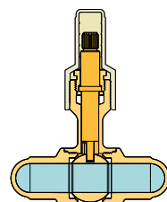
1690U
